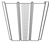
TRIPLE 4" CENTER-LANCED SOFFIT 4.4 Sq. In. / Sq. Ft.
