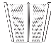
DOUBLE 6" FULLY-LANCED SOFFIT 10.6 Sq. In. / Sq. Ft.
