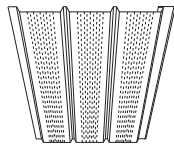
TRIPLE 4" FULLY-LANCED SOFFIT 13.2 Sq. In. / Sq. Ft.
