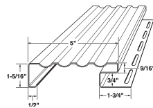
5" FLUTED LINEAL LINF5
