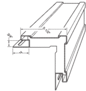
TRADITIONAL 5 1/2" OUTSIDE CORNER POST WITH FOAM INSERT TF0/P55
