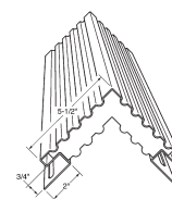
FLUTED 5 1/2" OUTSIDE CORNER POST FF0/P55
